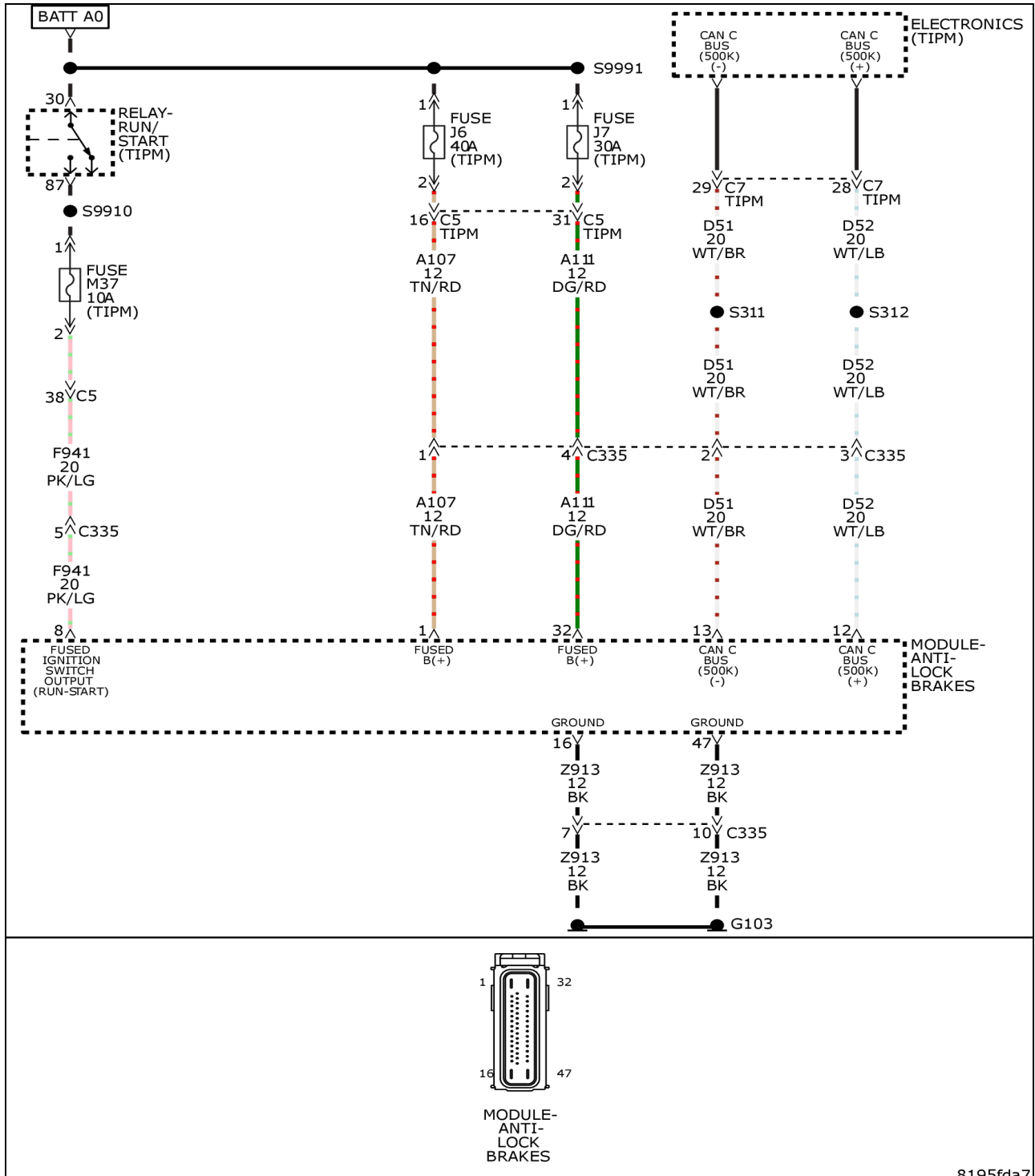
Fig 1: Antilock Brake Module (ABS) Wiring Diagram
